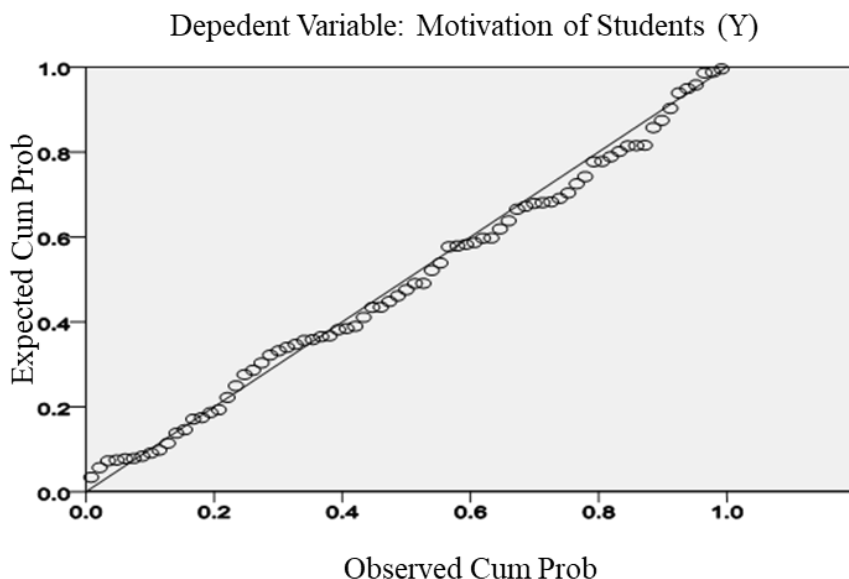
Figure: Normality test
