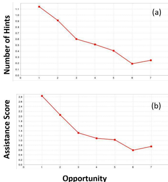
Figure 1. (a and b) Extent of assistance students need with successive opportunities and hints given by intelligent tutor
